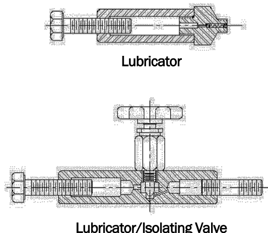
Figure 2: Optional Lubricator and Lubricator/Isolating Valve
